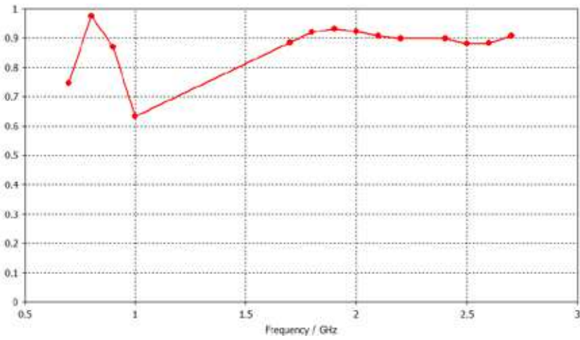
Typical Efficiency
